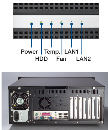
Rear view of ACP-4360MB
