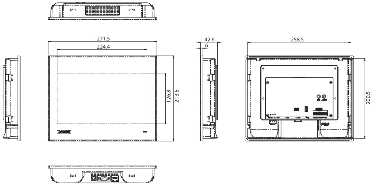
Panel Cut-out Dimensions: 260 x 201.5 mm (10.24" x 7.93")
