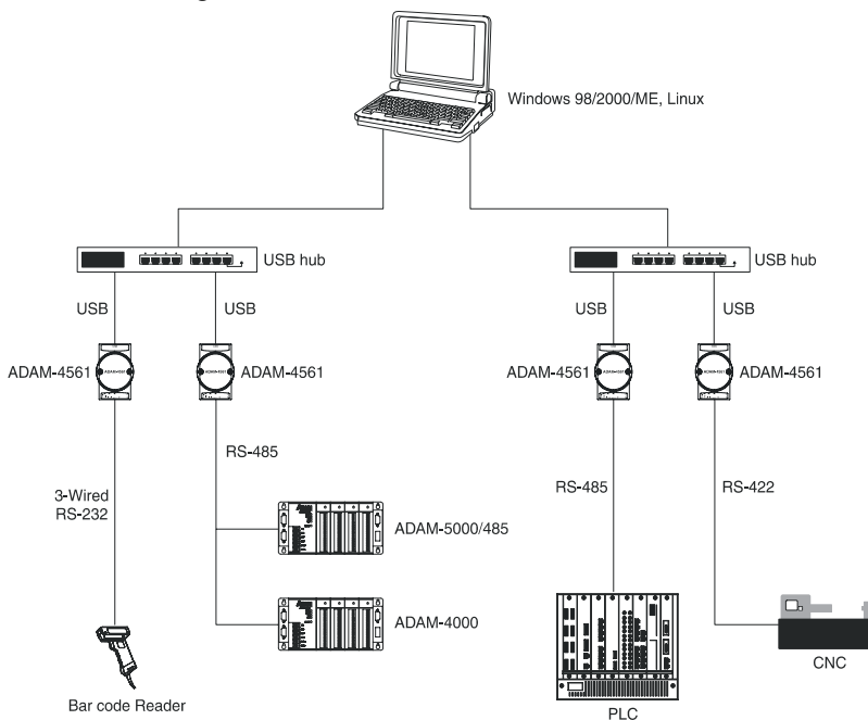
Figure 2.1: Network Architecture
