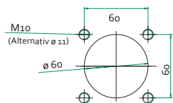
HLT Wandgelenk / Wall joint Art. Nr. / Part No.: 40102-01
